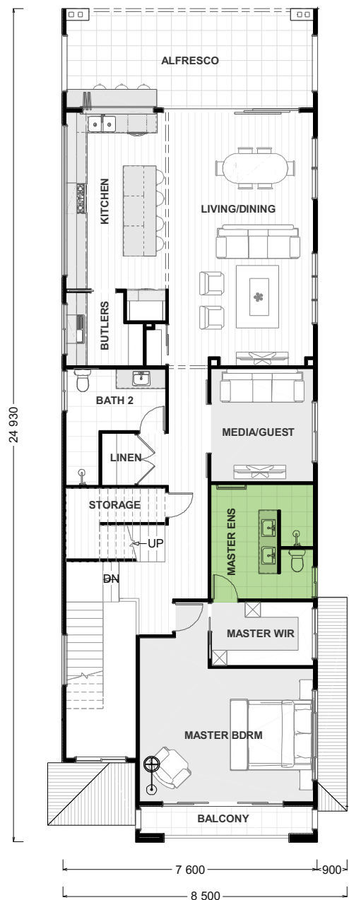
FIRST FLOOR
