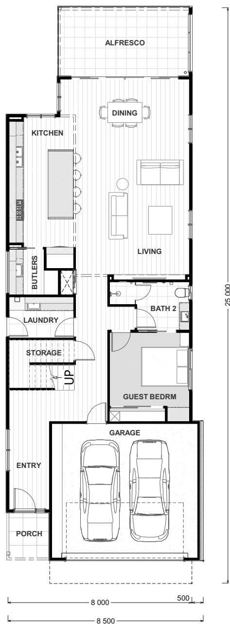
GROUND FLOOR
